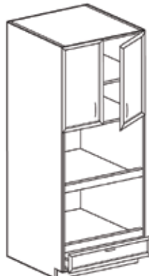
Double Oven Cabinets DO 30 96 24
